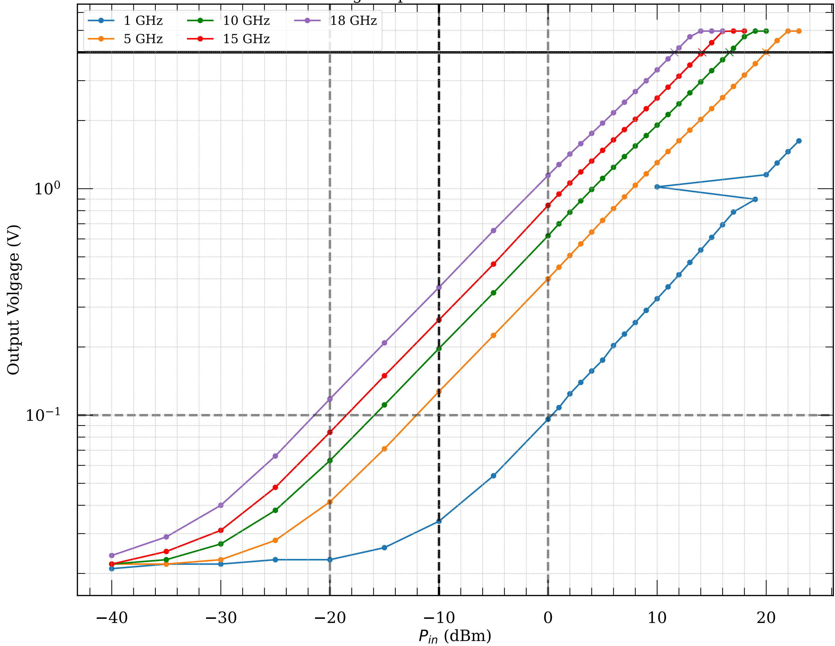
Measured voltage-to-power curve of detector module065
